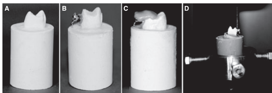
Fig. 1. (A) Die stone specimen. (B) Lingual bracket positioned on the die stone tooth. (C) Transference guide on the bracket and occlusal surface of the die stone tooth. (D) Specimen positioned in the MTS machine.
